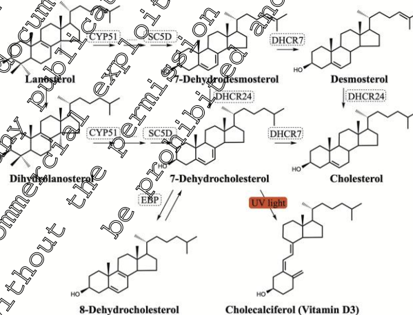
Figure CA 5.8.2/21-1: schematic of cholesterol biosynthesis
