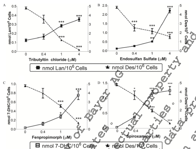
Figure CA 5.8.2/21-5: Concentration-dependent response of lead-hit compounds on intracellular levels of 7-dehydrocholesterol (D, open squares) and desmosterol (solid triangles) in Neuro-2a cells. Cells were exposed to (C) spiroxamine at the indicated concentration for 24 h. Data presented as nmol sterol/million cells ( n=4 , \pm SEM). * p<0.05 , *** p<0.001 as determined by post hoc Dunnett's test following one-way ANOVA, using vehicle as the control comparison.
